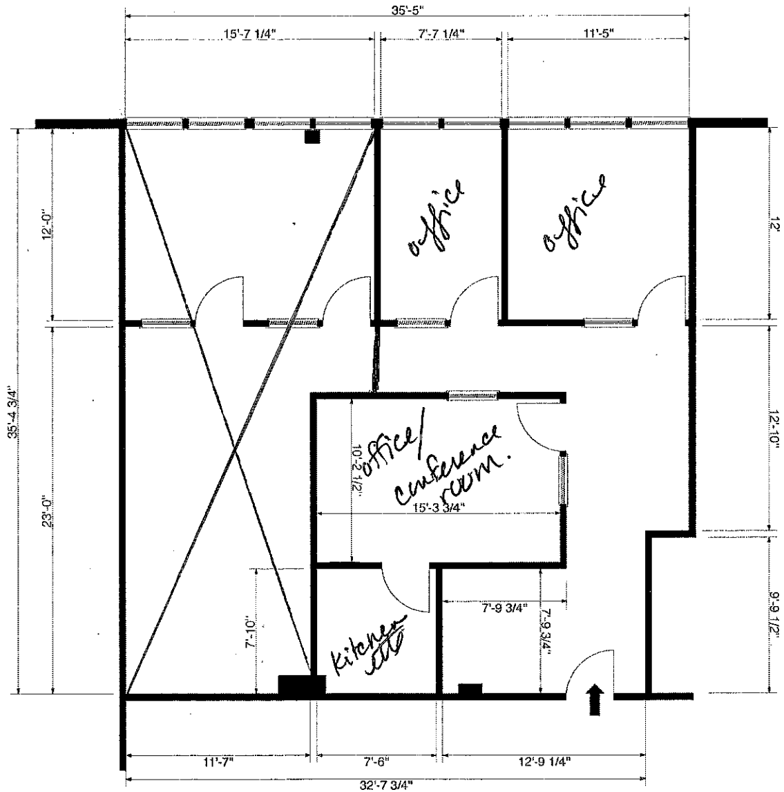
FLOOR PLAN 1/8" = 1' 0"
