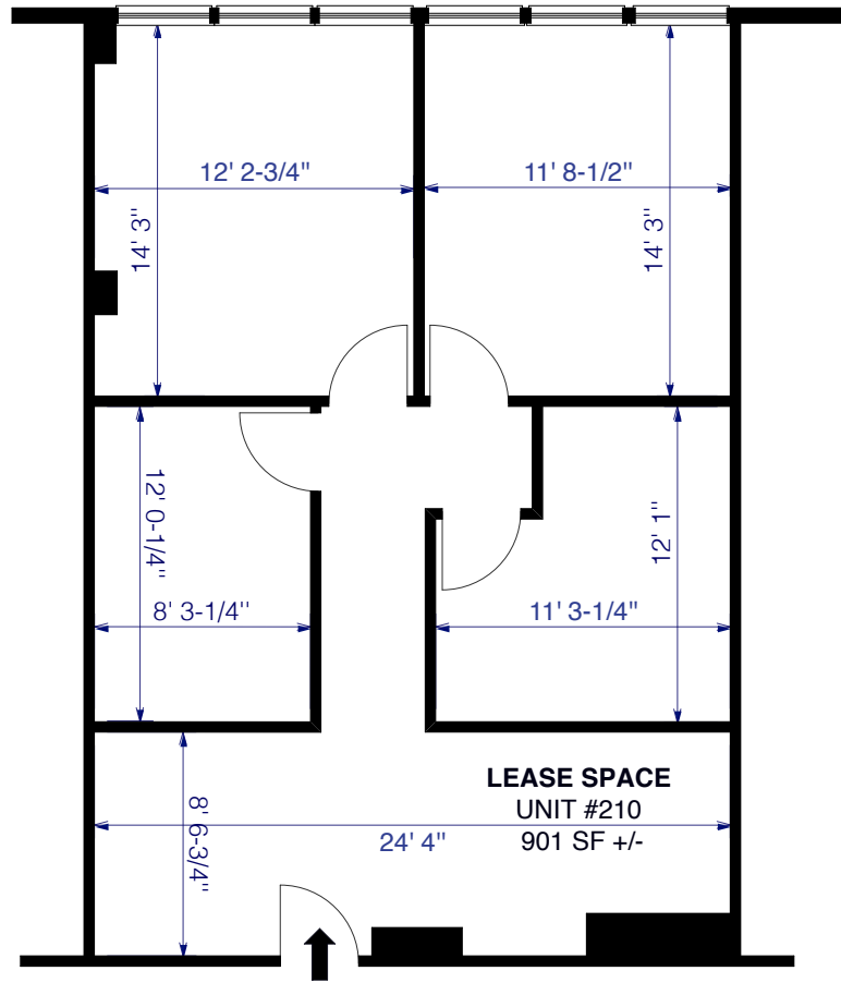
FLOOR PLAN 1/8" = 1' 0"
