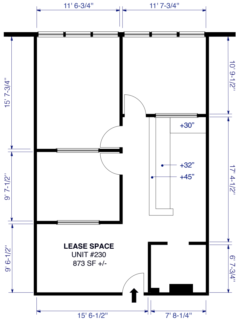
FLOOR PLAN 1/8" = 1' 0"
